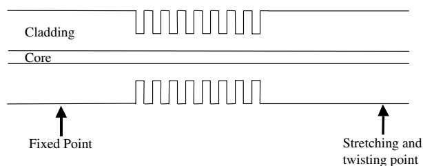
Figure 4. Corrugated fibre LPG.
