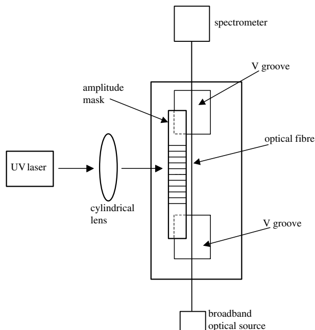
Figure 3. LPG fabrication using a UV laser.
