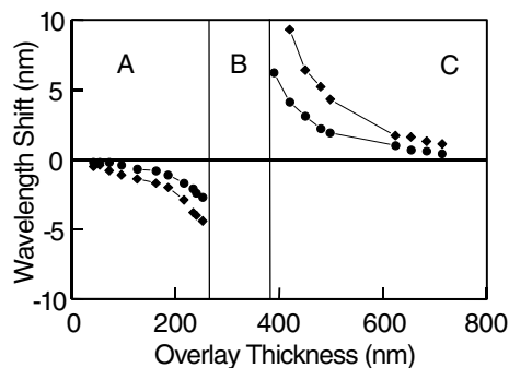
Figure 10. Experimentally determined response of two of the attenuation bands of an LPG to the deposition of a thin film of material of refractive index 1.57. (From [80].)
