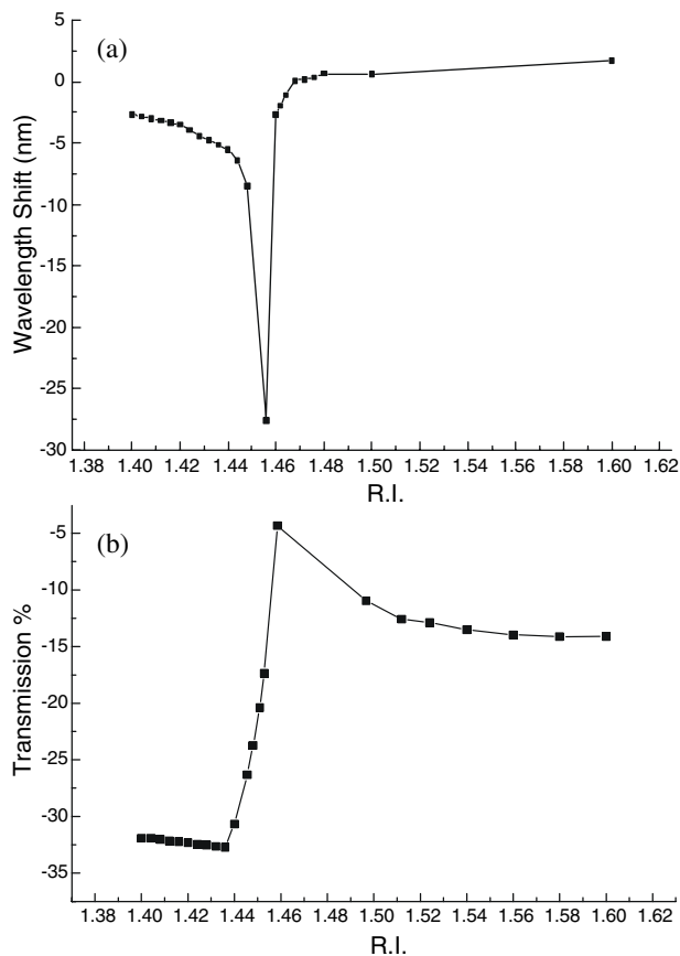
Figure 9. Plot of (a) the wavelength shift and (b) the minimum transmission value of an attenuation band against the RI of the material surrounding the LPG of period 400 \mu\text{m} written in boron–germanium co-doped fibre with cut off wavelength 650 \text{ nm} . (From [55].)
