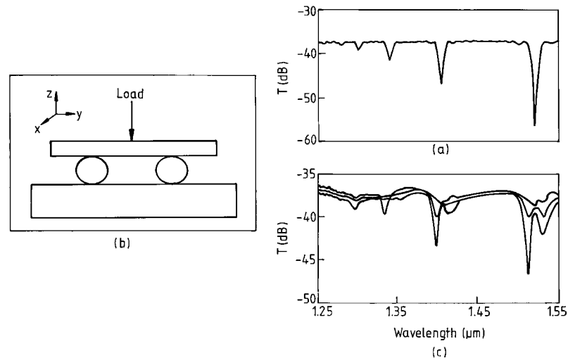
Figure 8. Loading system and transmission spectra of an LPG of period 490 \mu\text{m} , written in B–Ge co-doped fibre, unloaded and loaded, showing the generation of attenuation band splitting resulting from the induced birefringence. (After [64].)
